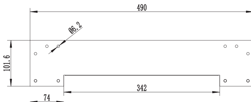
BACK
