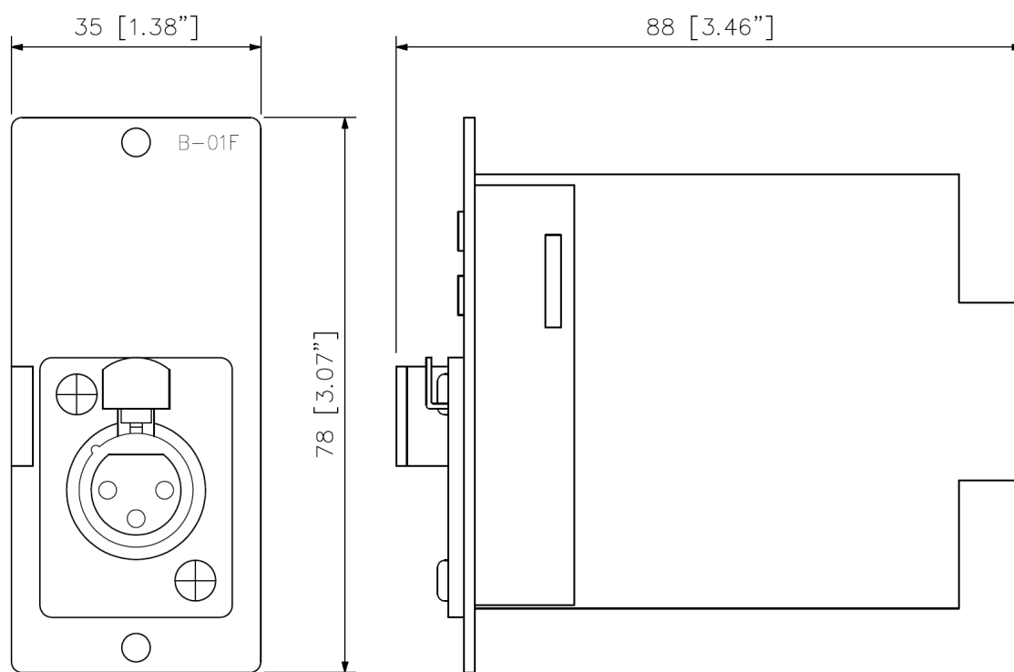
Front View
