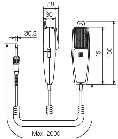
Accessory microphone (1/5)
