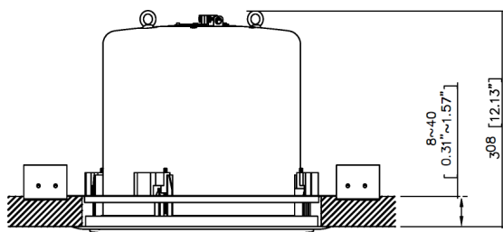
[CEILING MOUNTING]
