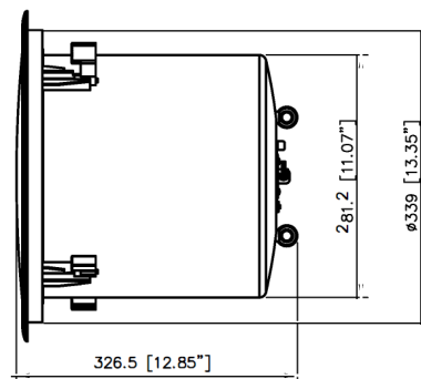
[CEILING MOUNTING]
