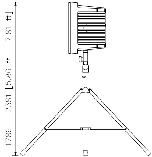
ST-34B (option) mounting
