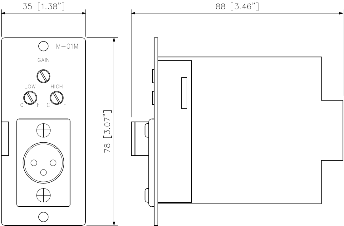
Front View
