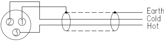
Connection Diagram
