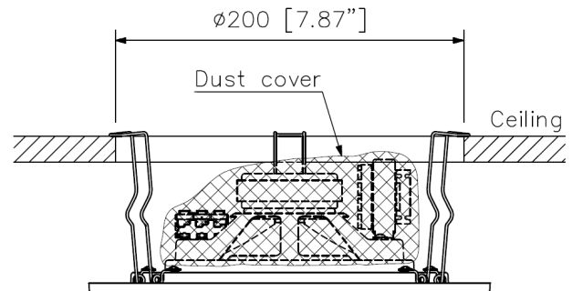
Mounting Diagram
