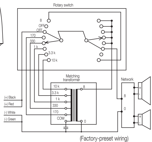
Wiring Diagram
