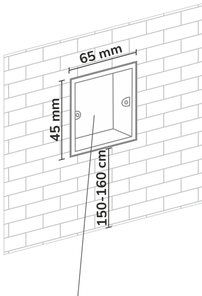
Mounting box
