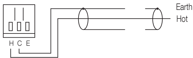
Connection Diagram
